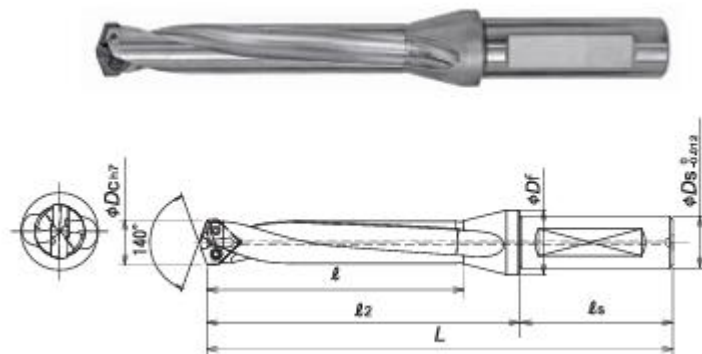
TEZDF-MS type ( L/D=3 )
