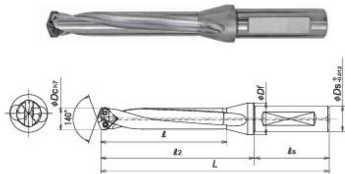
TEZDF-ML type (L/D=5)
